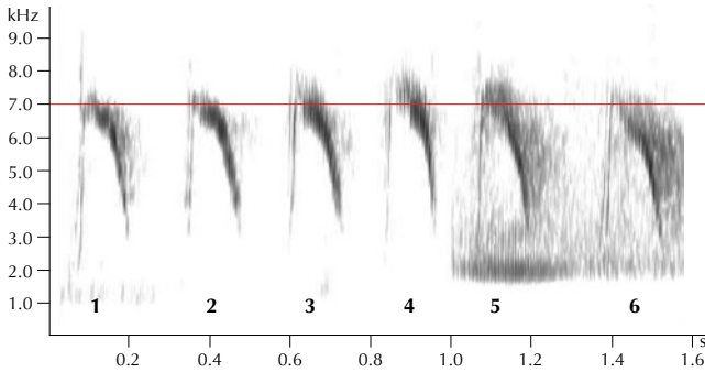
FIGURE 8 Flight calls of taxa belonging to eastern group: 1 Manchurian Wagtail / Mantsjoerijse Kwikstaart Motacilla macronyx , Kiat Ngong, Laos, 20 December 2008 (Wouter Halfwerk; XC27241); 2-3 Manchurian Wagtail / Mantsjoerijse Kwikstaart Motacilla macronyx , Phnom Krom marsh, Siem Reap, Cambodia, 13 March 2013 (Frank Lambert; XC127900, XC127898); 4-5 Green-headed Wagtail / Groenkopkwikstaart Motacilla taivana , Shanhua, Taiwan, 21 February 2008 (Sander Bot; XC65415, XC65416). Horizontal line at 7 kHz added to facilitate comparison of flight calls. Note ascending part 1 is quite similar to north-western group but spacing between both lines of part 1 slightly different: close together at lowest pitch but widening with increasing pitch. Part 2 resembles south-western group; however, note absence of distinct hook in first part.
